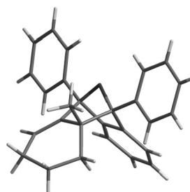
Figure 3. X-ray structure of compound endo - 24 .
