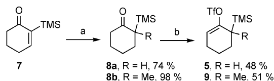
Scheme 2. Synthesis of 1,2-cyclohexadiene precursors. Reagents and conditions: (a) i. L-Selectride, ii. \text{NH}_4\text{Cl} (aq.) for 8a or MeI for 8b ; (b) i. LDA ii. \text{PhNTf}_2 .
