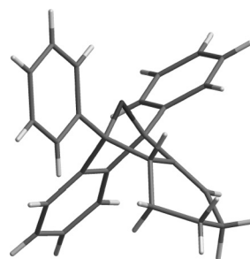
Figure 1. X-ray structure of compound endo - 14 .
