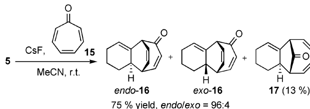
Scheme 5. Cycloadditions of 1,2-cyclohexadiene with tropone.
