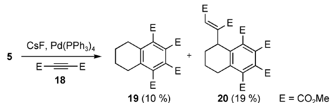
Scheme 6. Pd-promoted reaction of 1,2-cyclohexadiene with dimethyl acetylenedicarboxylate.
