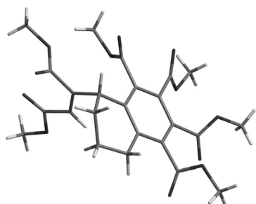
Figure 2. X-ray structure of compound 20 .
