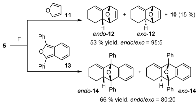
Scheme 4. [4+2] Cycloaddition reactions of 1,2-cyclohexadiene.
