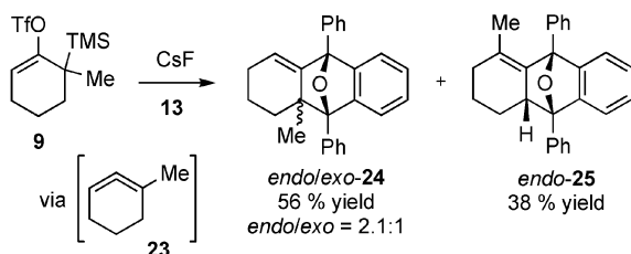
Scheme 8. [4+2] Cycloaddition reaction of cyclic allene 23 .
